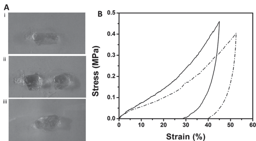
Figure 5. Self-healing of a MiGel. A-i) Picture of a virgin MiGel (10% w/v), A-ii) the MiGel after it has been severed into two pieces, and A-iii) the repaired MiGel about 1 min after the two pieces are put back together. B) Compressive stress response of the virgin (solid) and healed (dashed) MiGel (10% w/v).
