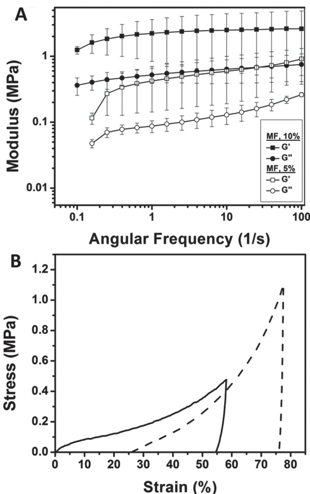
Figure 4. Mechanical characterization of MiGels. A) Storage and loss modulus for MiGels at 25 °C for two polymer concentrations (10% w/v, 5% w/v). Each point on the plot is an average value of three independent measurements and error bars are calculated standard deviations of the three measurements. B) Cyclic compression and expansion tests for MiGels (10% w/v) at 25 °C from 0% to 55% (solid line) and then immediately from 25% to 75% compressive strain (dashed line).
