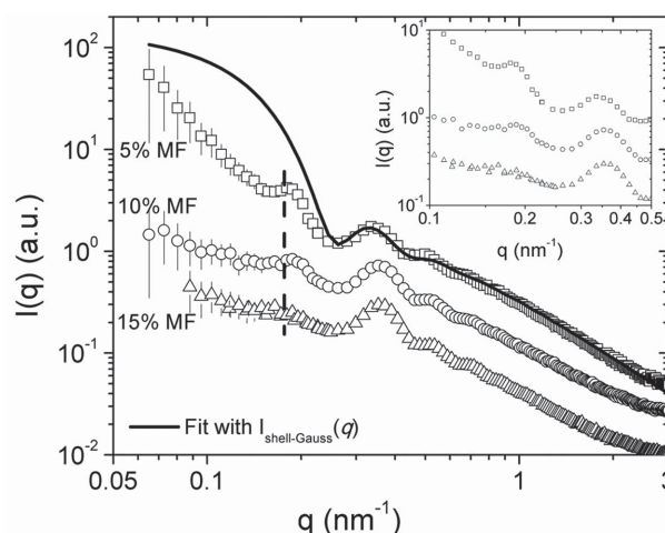
Figure 3. SAXS intensity profiles for MiGels formed at three different concentrations of MF-ELP. Squares: 5% w/v MiGel, circles: 10% w/v MiGel, triangles: 15% w/v MiGel; the data are offset for clarity of presentation. The solid black line represents the fit to 5% w/v MiGel SAXS profile at q > 0.3\ \text{nm}^{-1} using the form factor of spherical shells and Gaussian chains ( I_{\text{shell-Gauss}} ). The dashed line is a reference to indicate the shift in the inter-particle correlation peak for three gel concentrations (also shown as the inset).
